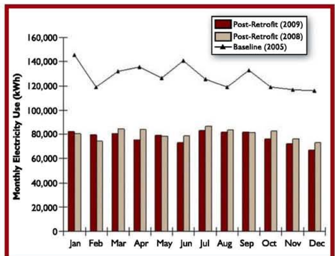
Figure 3: Monthly pre- and post-retrofit electricity consumption.
