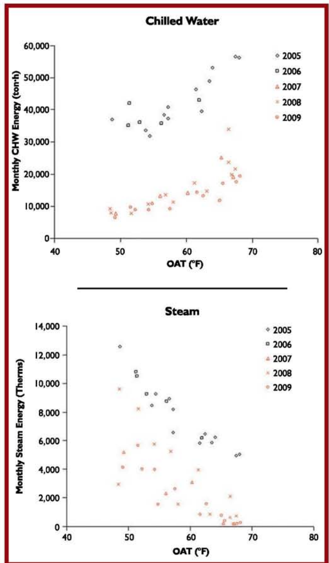
Figure 2: Pre- and post-retrofit chilled water and steam consumption.
