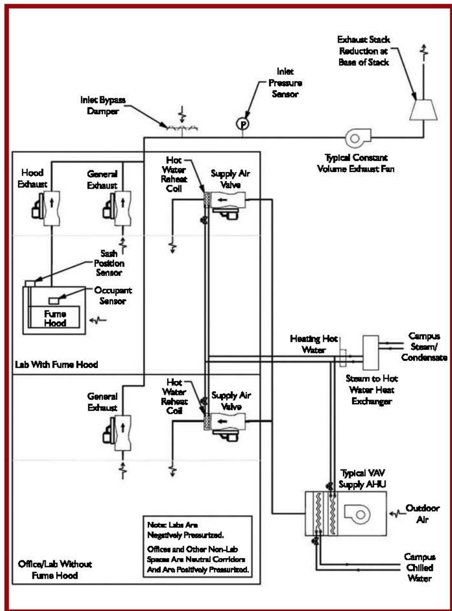
Figure 1: Stauffer I chemistry laboratory VAV retrofit system.
